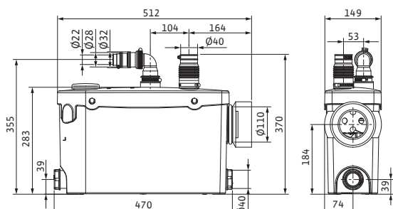
Wilo-HiSewlift 3-I35
