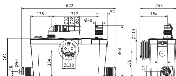
Wilo-HiSewlift 3-35
