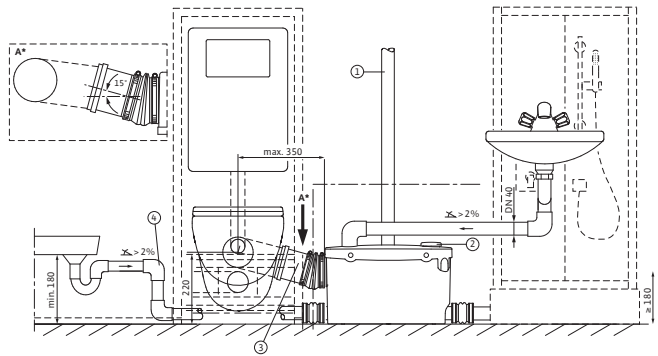
Wilo-HiSewlift 3-I35
