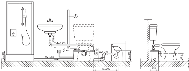
Wilo-HiSewlift 3-35
